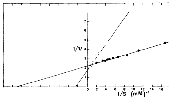
Fig.2. Lineweaver-Burk plot of the activity of X-prolyl dipeptidyl aminopeptidase against L-alanyl-L-proline- p -nitroanilide concentration. The enzymatic activity was measured at 37°C in 100 mM Hepes-Tris buffer (pH 7.0) and expressed as the increase in absorbance at 405 nm. (○—○) Heat-resistant X-prolyl DPAPase (protoplast lysate preincubated prior to substrate addition at 60°C for 30 min). K_m app., 0.4 mM. (●—●) Heat-labile X-prolyl DPAPase (purified vacuolar membranes). K_m app., 0.06 mM.
